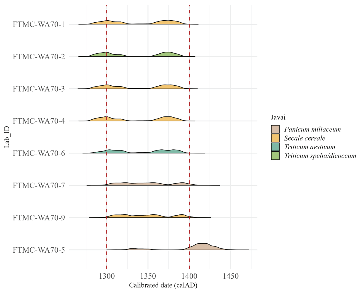
Fig. 2. A calibration plot of ^{14}\text{C} dates obtained for charred plant remains from outer bailey of Merkinė hillfort.
